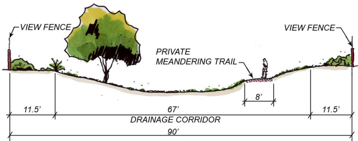
Initial Concept for the Laveen Drainageway
